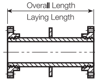
Flange-Thrust Collar-Flange
